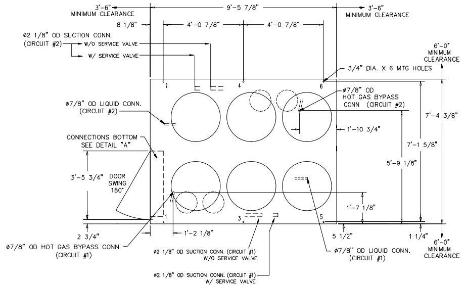
Figure DD-6 –Air-Cooled Condensing Unit –RAUC 60Ton
